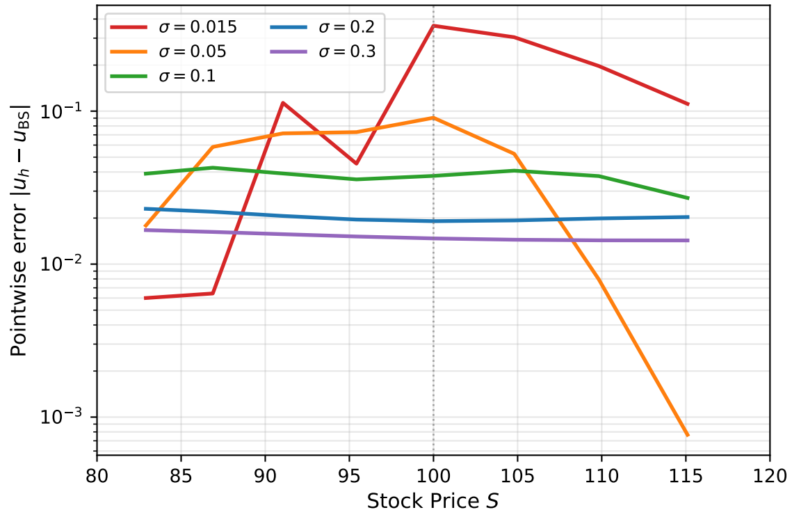
Pointwise error by volatility (convection-dominated regime at low \sigma )
