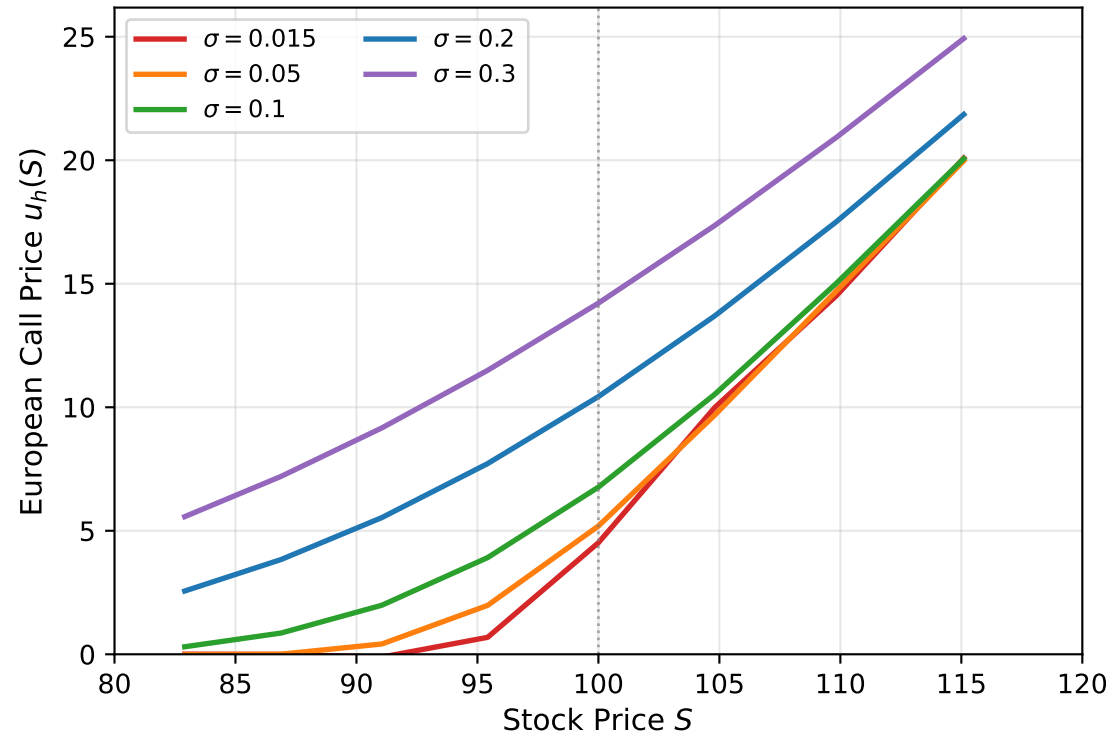
V1 primal DPG: stability across volatility regimes ( N_x = 128 , N_t = 1000 , K = 100 , T = 1 , r = 0.05 )
