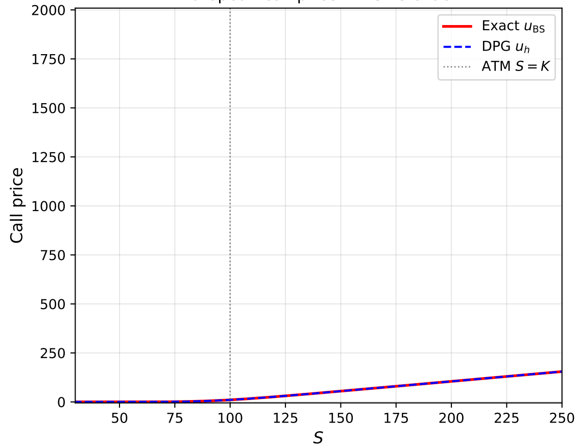
European call price: DPG vs exact
