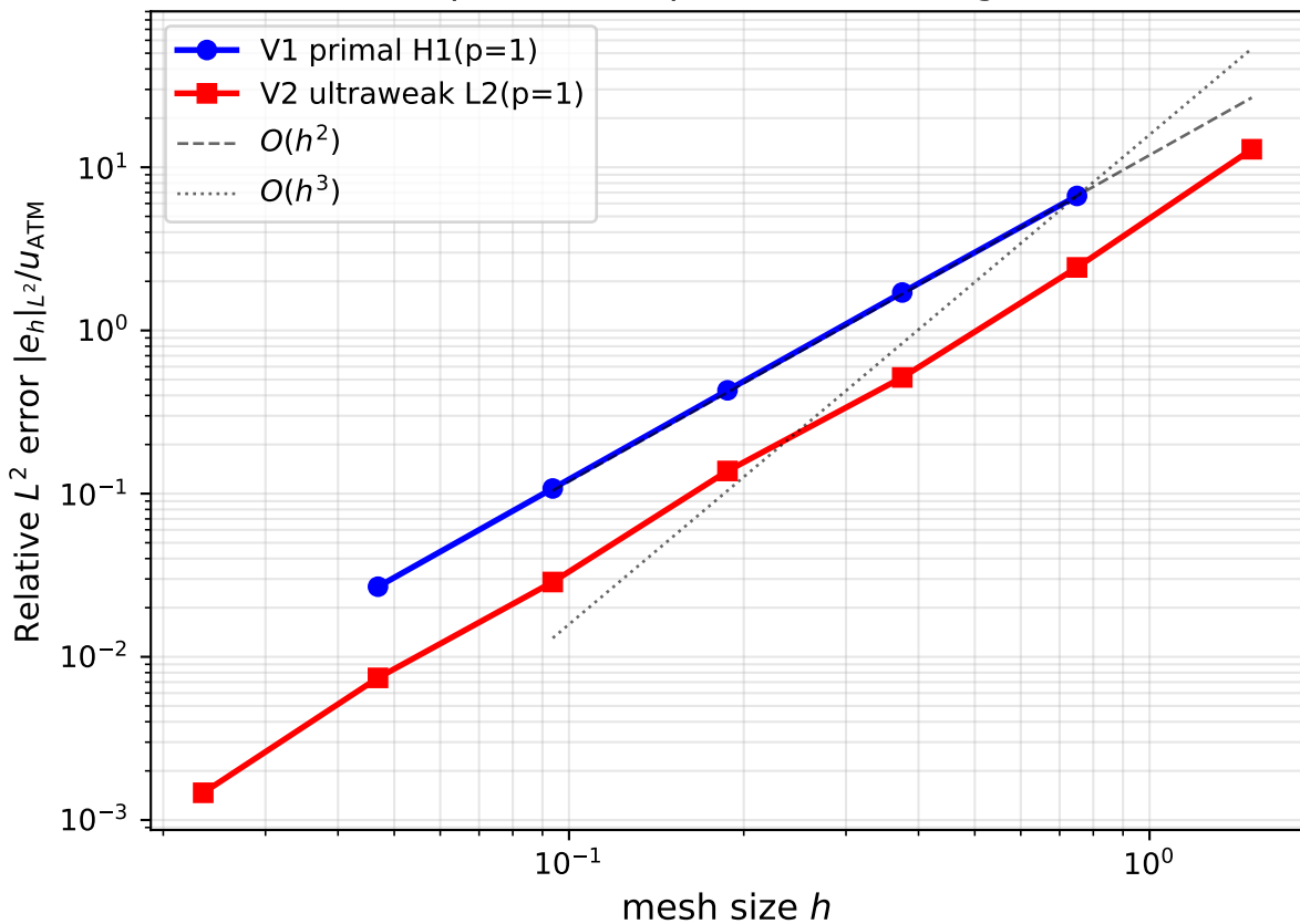
European call: spatial L^2 convergence
