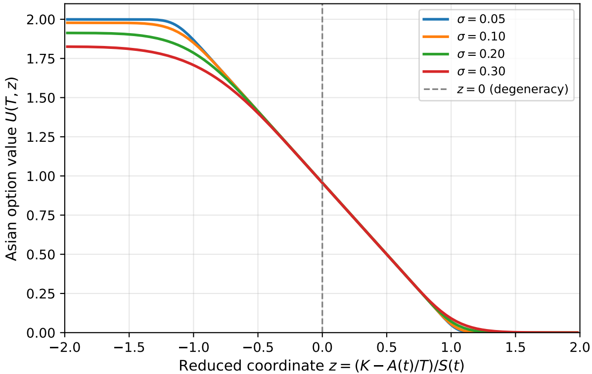
Asian Call Option — DPG Solution (Rogers-Shi Reduction)
