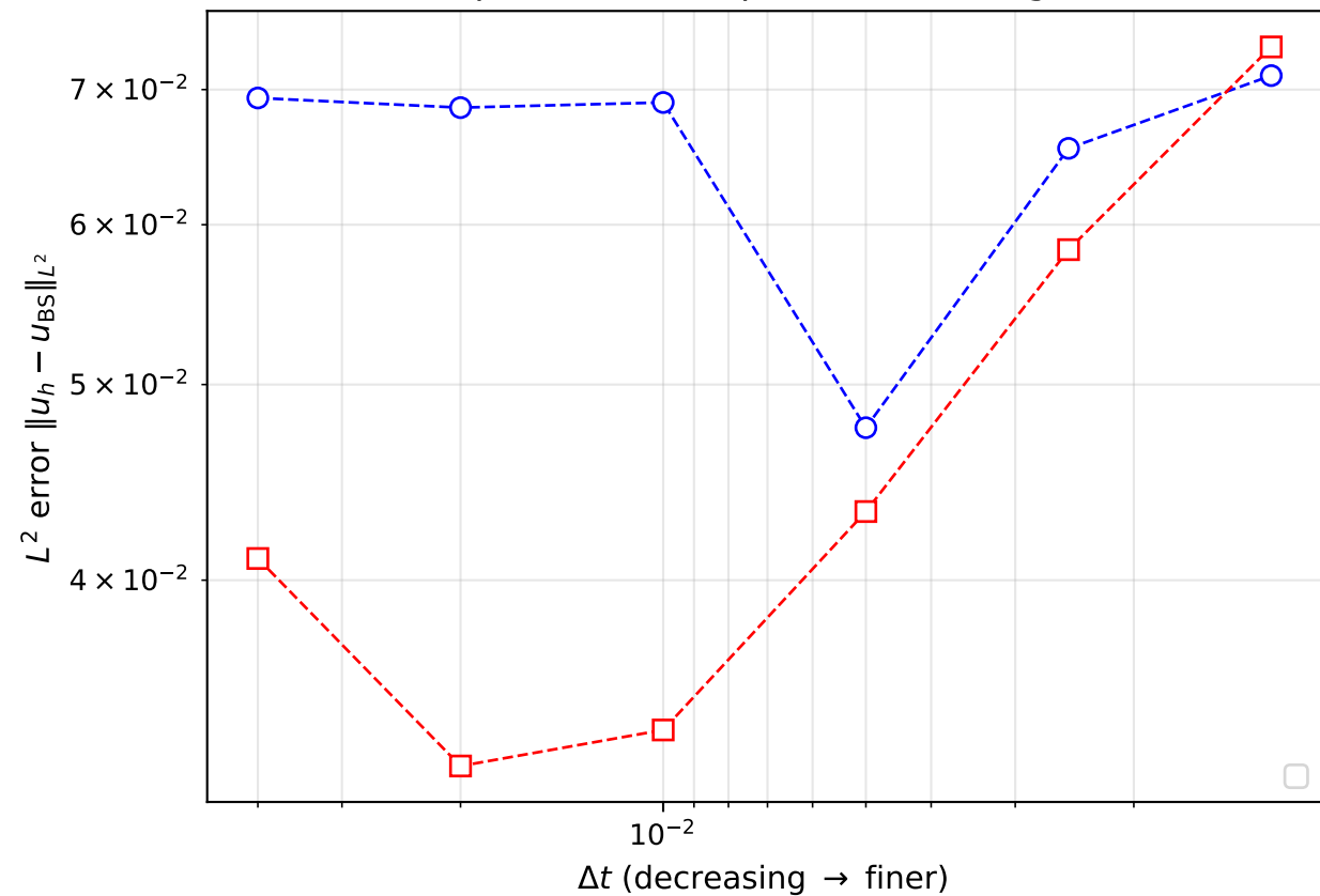
European call: temporal L^2 convergence
