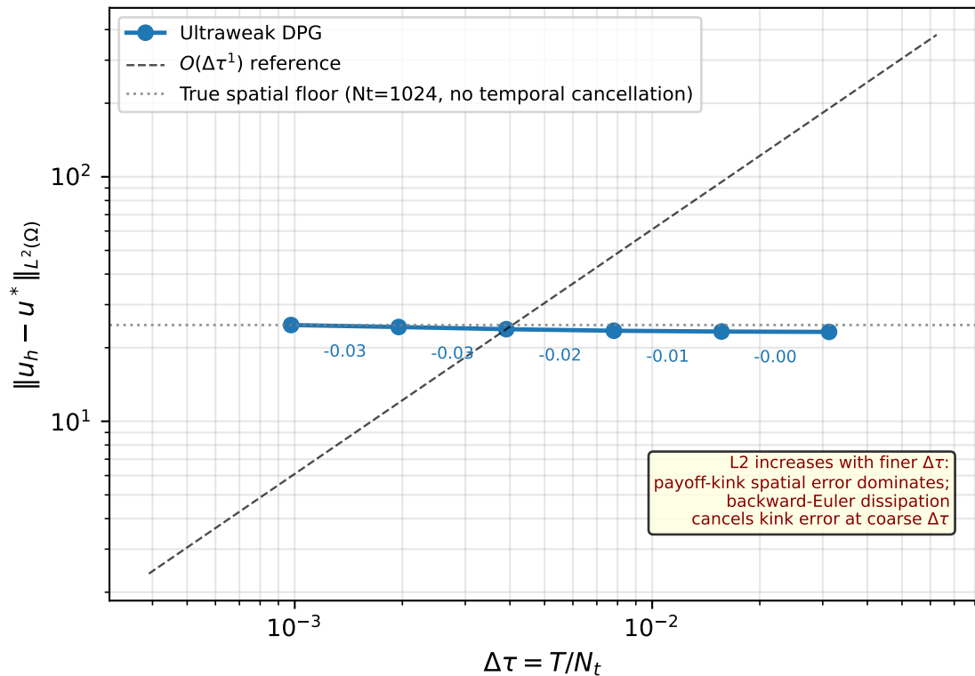
Best-of call (Stulz): temporal study, N = 384 , \rho = 0.5 [error cancellation]
