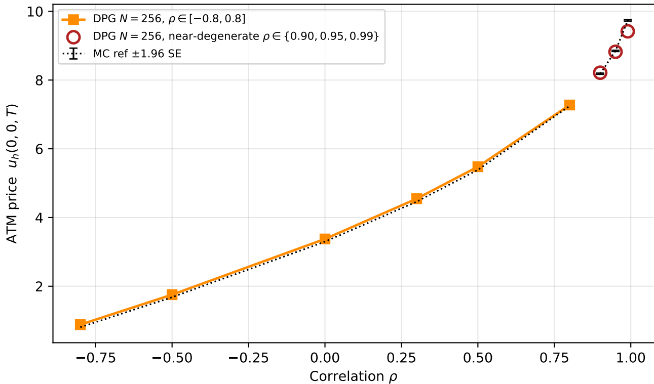
Basket call-on-min: price vs \rho (incl. near-degenerate)
