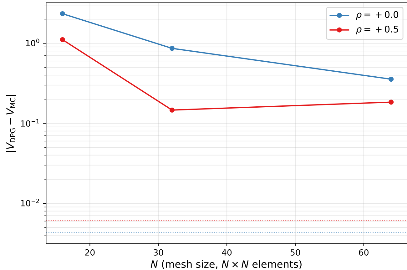
Basket spatial refinement at ATM ( S_1 = S_2 = K = 100 )
