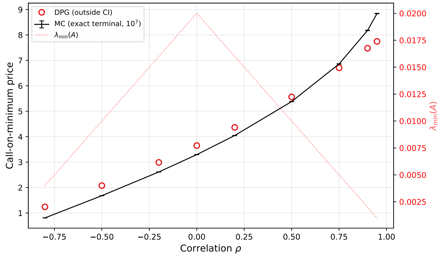
DPG vs MC: call-on-minimum, K = 100 , T = 1 , N = 64
