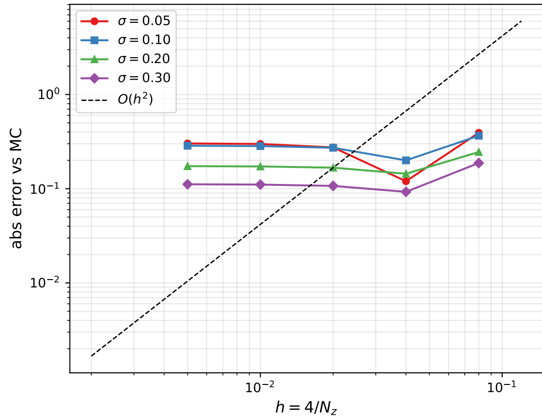
Asian spatial refinement, ATM K = 100 , N_t = 800
