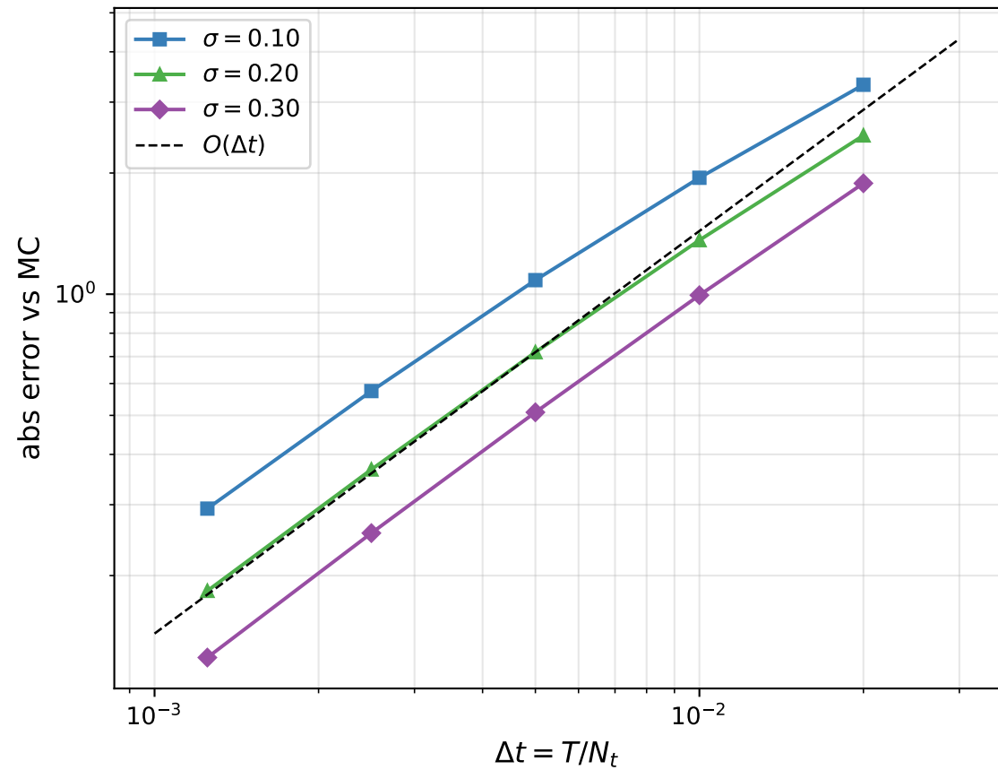
Asian temporal refinement, ATM K = 100 , N_z = 800
