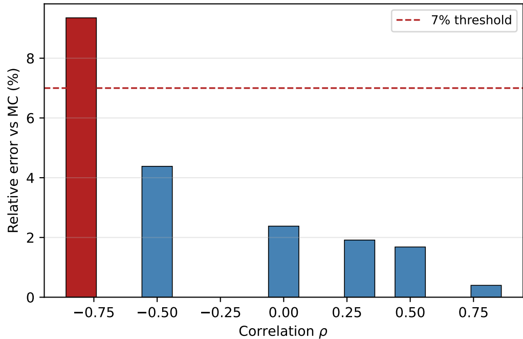
Price error vs \rho at N = 256
