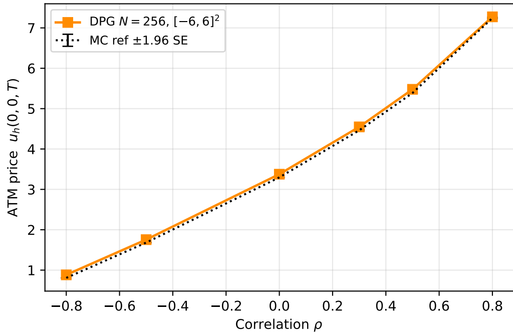
Basket call-on-min: price vs \rho
