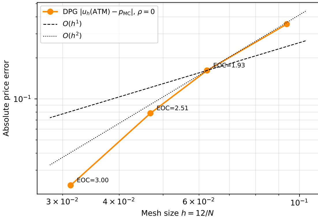
Basket call-on-min convergence, \rho = 0
