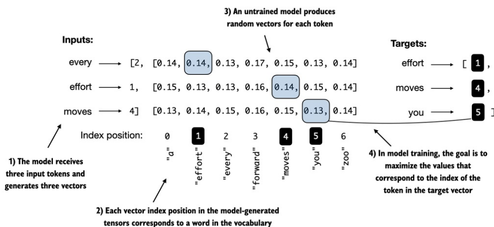
Figure 5.6 Before training, the model produces random next-token probability vectors. The goal of model training is to ensure that the probability values corresponding to the highlighted target token IDs are maximized.
