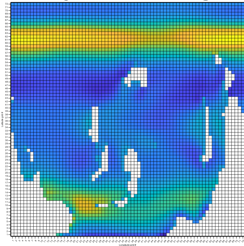
Data grid: wind stress out -- x @ u
