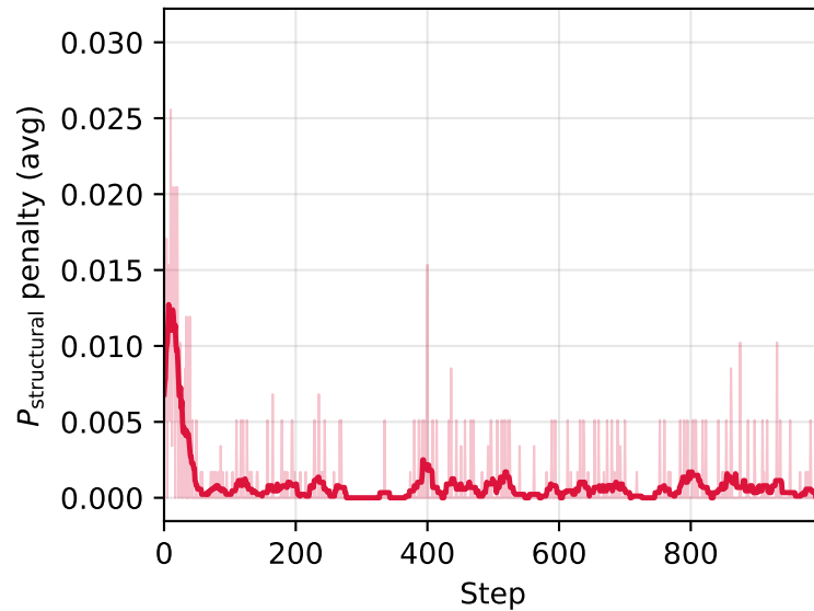
Reward Components (Fair-RLVR)
