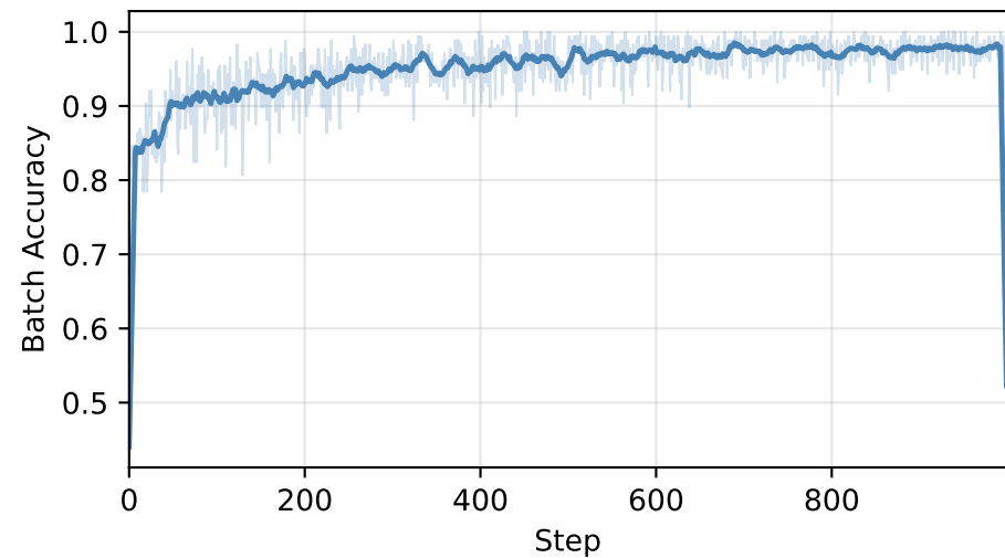
Training Trajectory (Fair-RLVR, \lambda = 0.5 )
