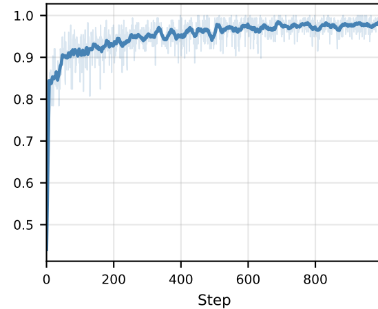
Batch Accuracy
