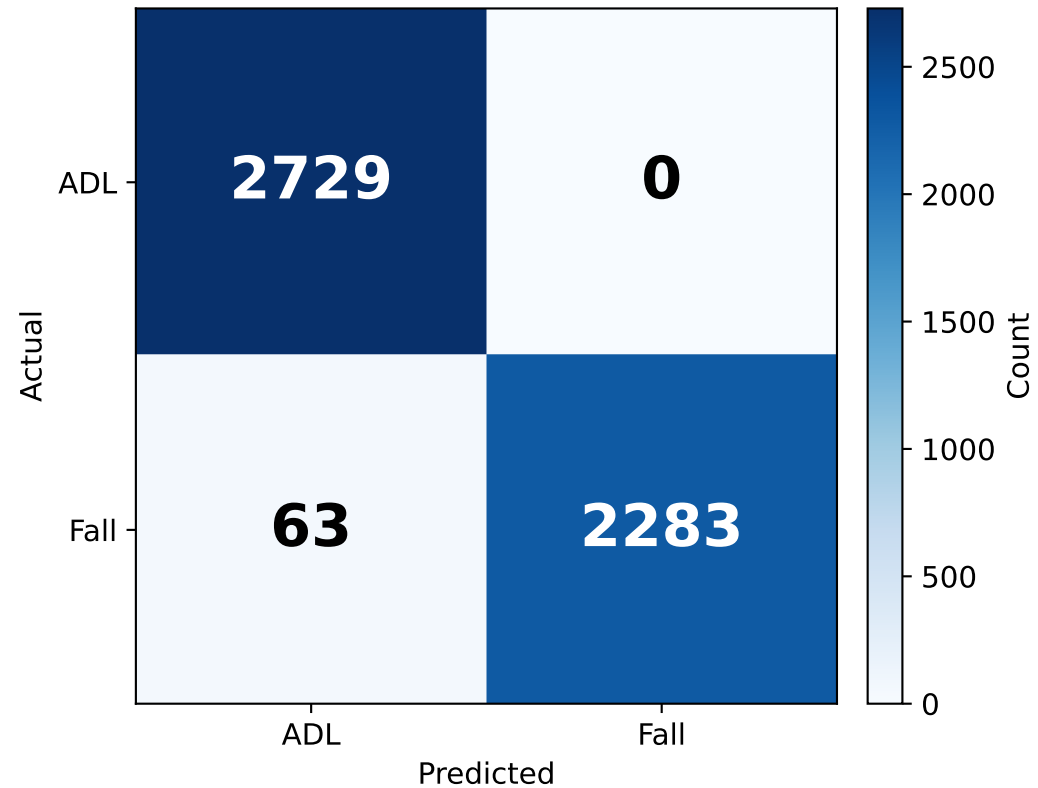
(b) KFall — ADXL+ITG + KNN (zero-shot, 5,075 events)
