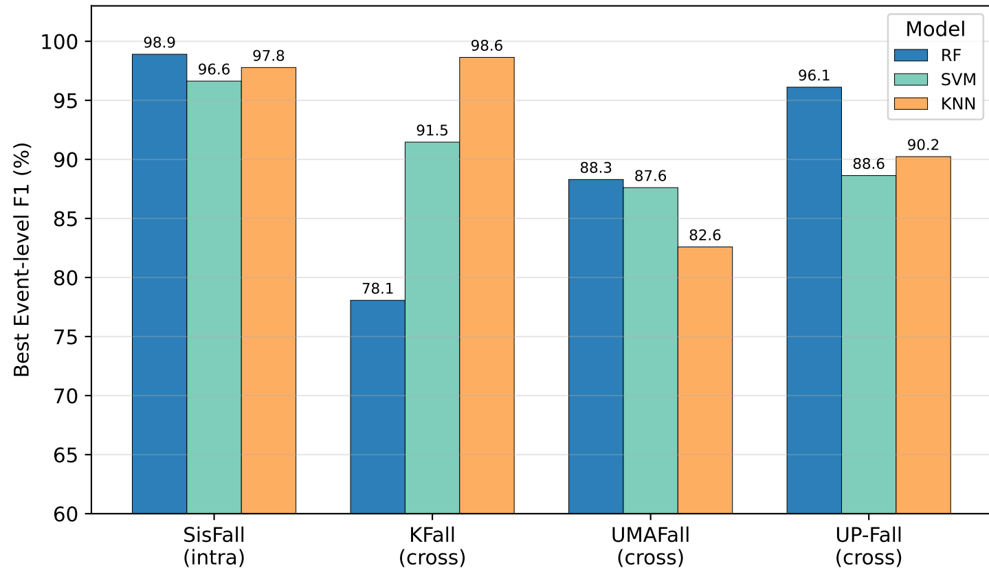
Cross-Dataset Generalization (best ML per dataset)
