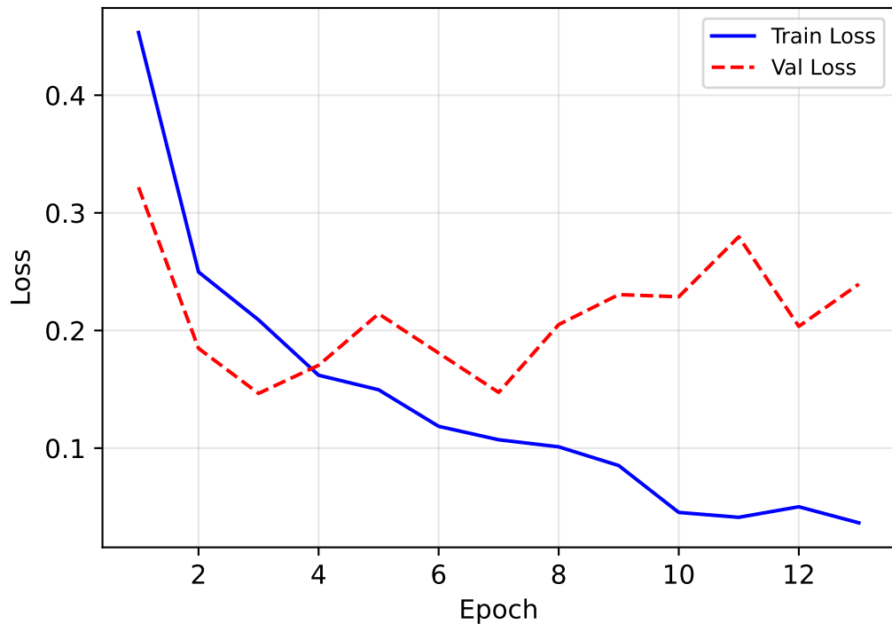
(a) Training & Validation Loss
