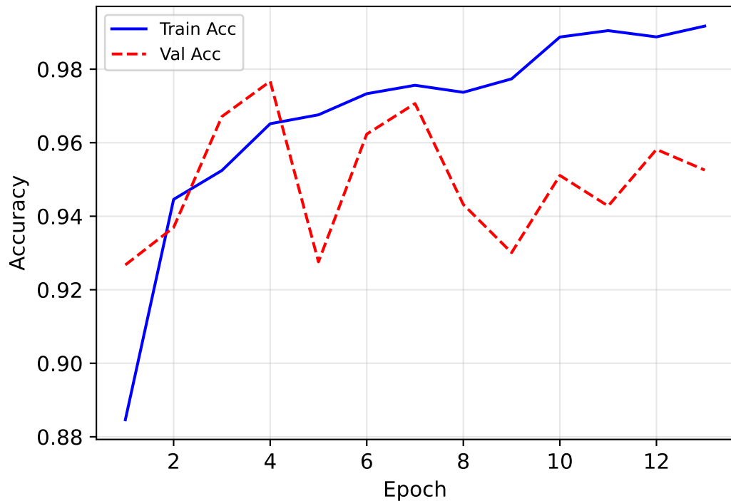
(b) Training & Validation Accuracy
