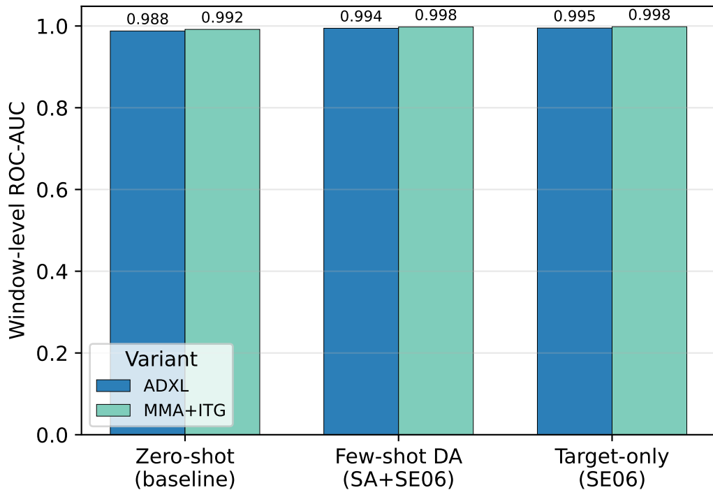
Window-level ROC-AUC
