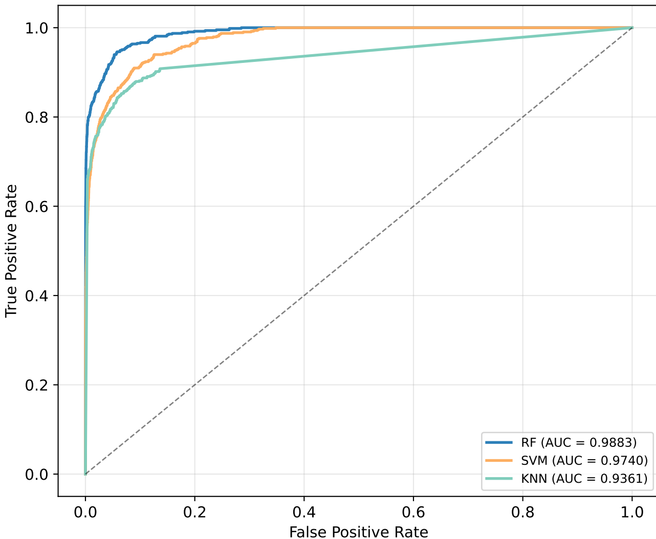
ROC Curves — ML Models on ADXL Test Set (Window-level)
