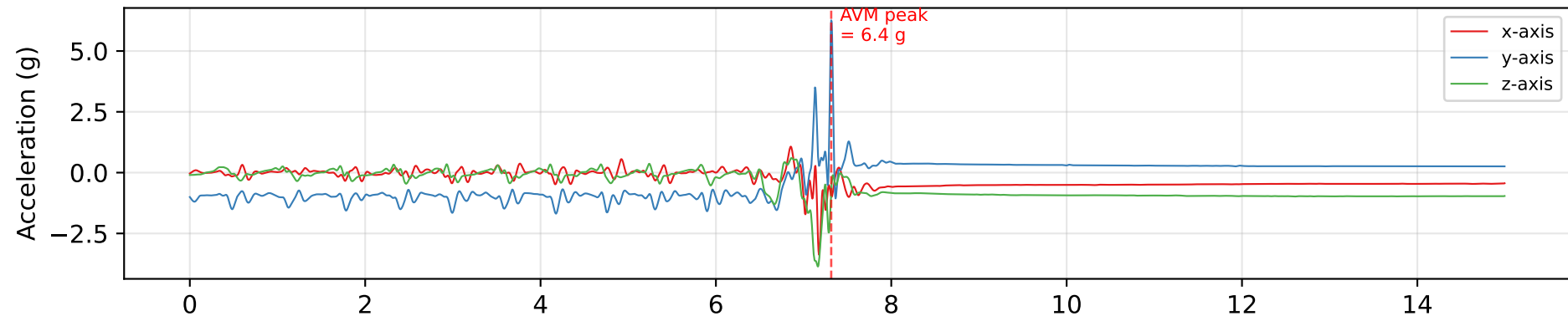
(a) Fall Event (F01 — Forward Fall)
