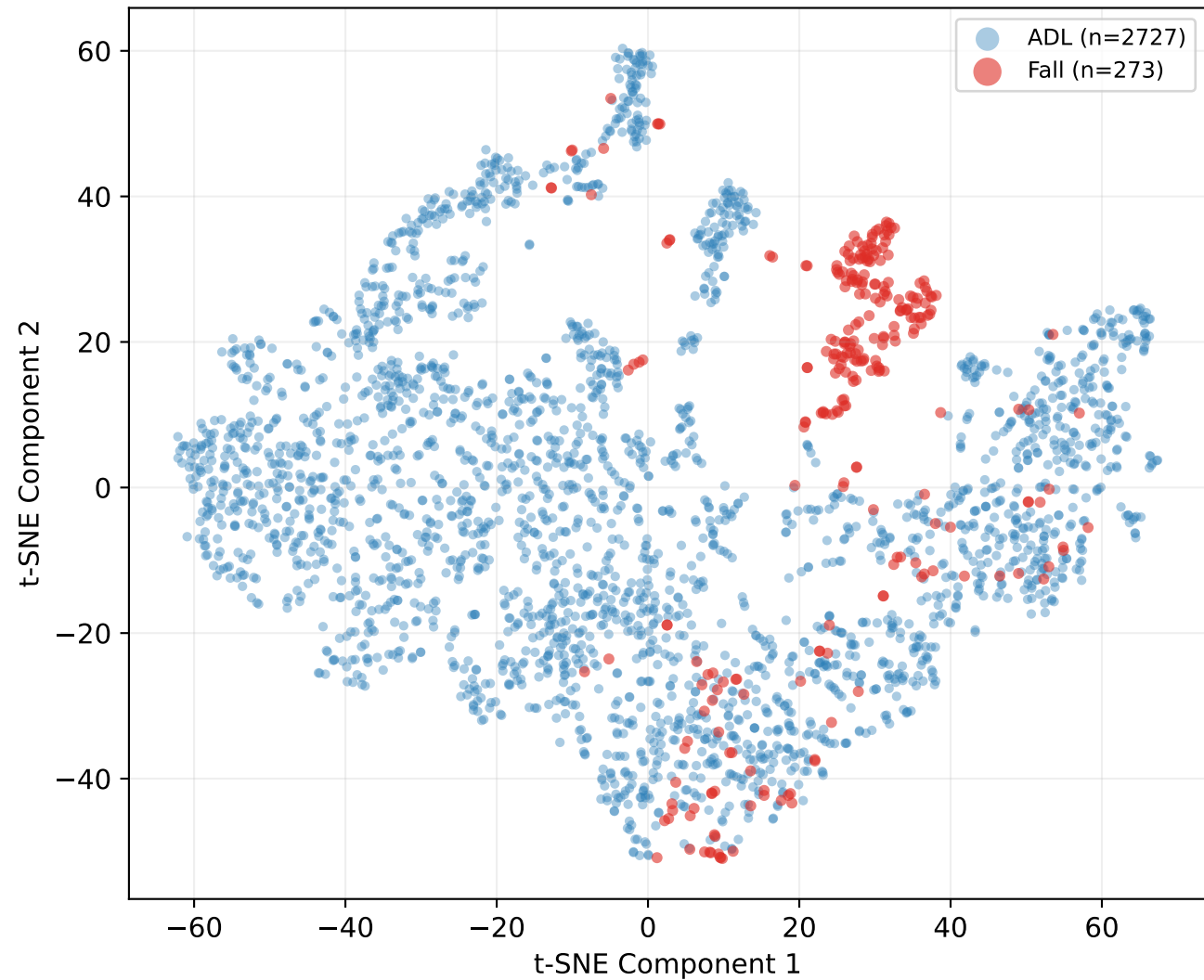
t-SNE Visualization of Extracted Features (ADXL, 54 features)
