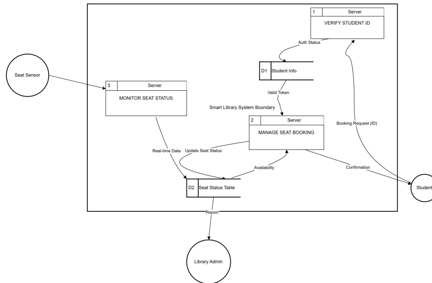
Figure 2. Level 1 DFD decomposing the system into primary functional processes.
