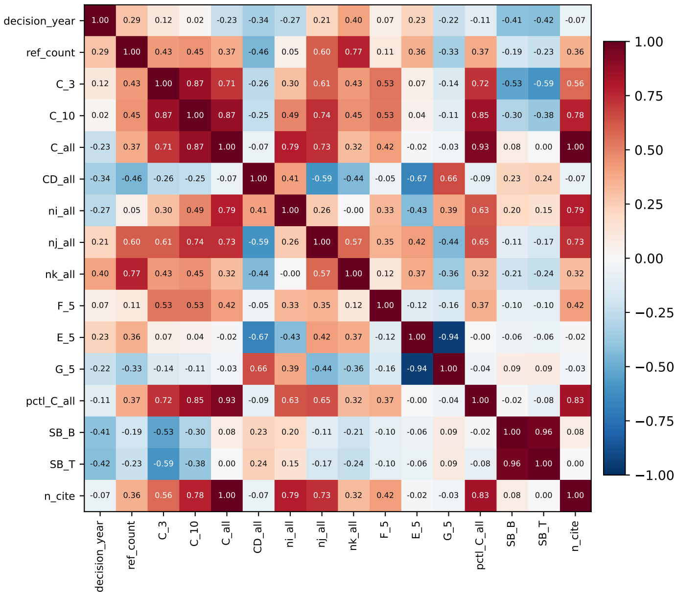
Spearman correlations (500k sample)
