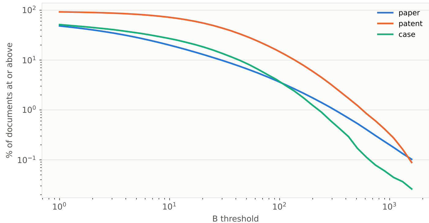
Survival of the beauty coefficient ( n_{\text{cite}} \geq 100 )
