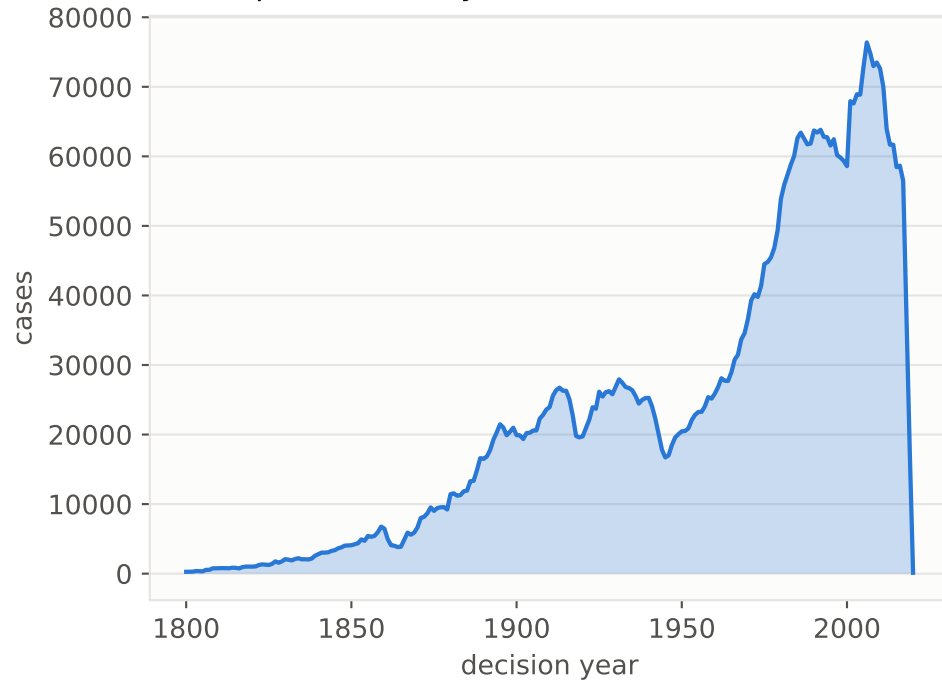
Cases per decision year
