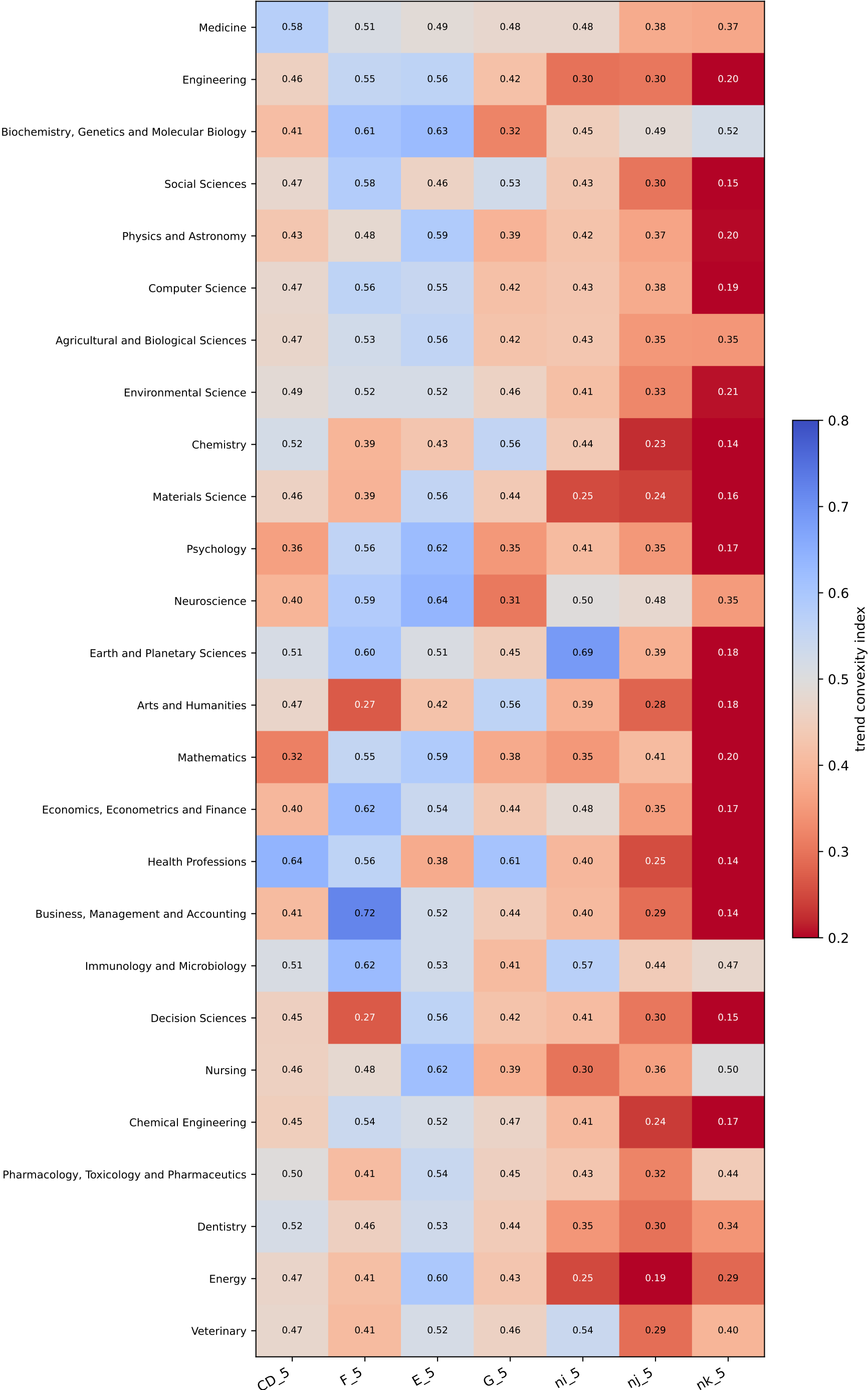
Yearly-trend convexity index: FoS x metric (<0.5 convex=red / >0.5 concave=blue)
