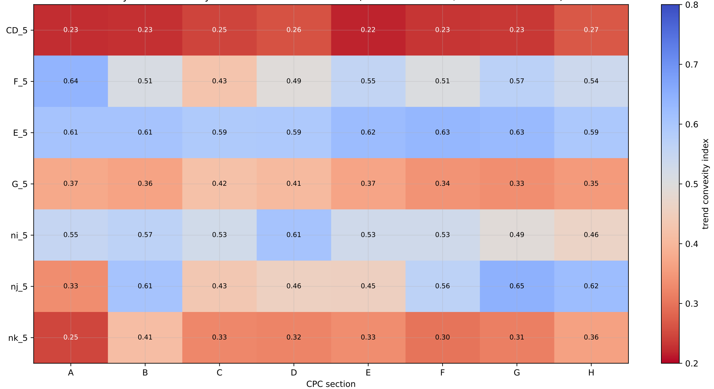
Yearly-trend convexity index: metric x CPC section (<0.5 convex=red / >0.5 concave=blue)
