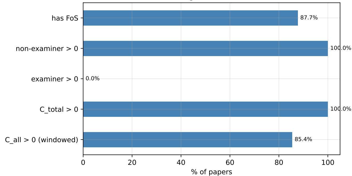
Coverage (N=5,106,527)
