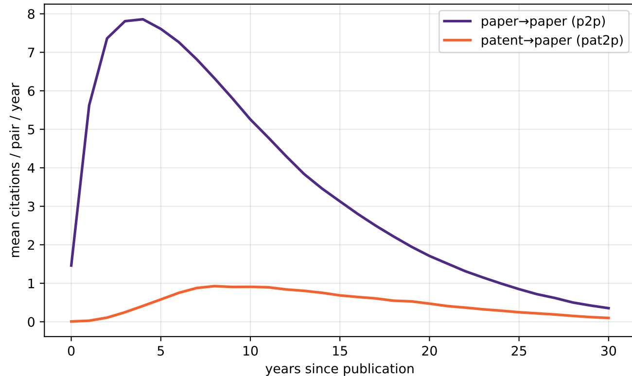
Paper-side citation-age profile
