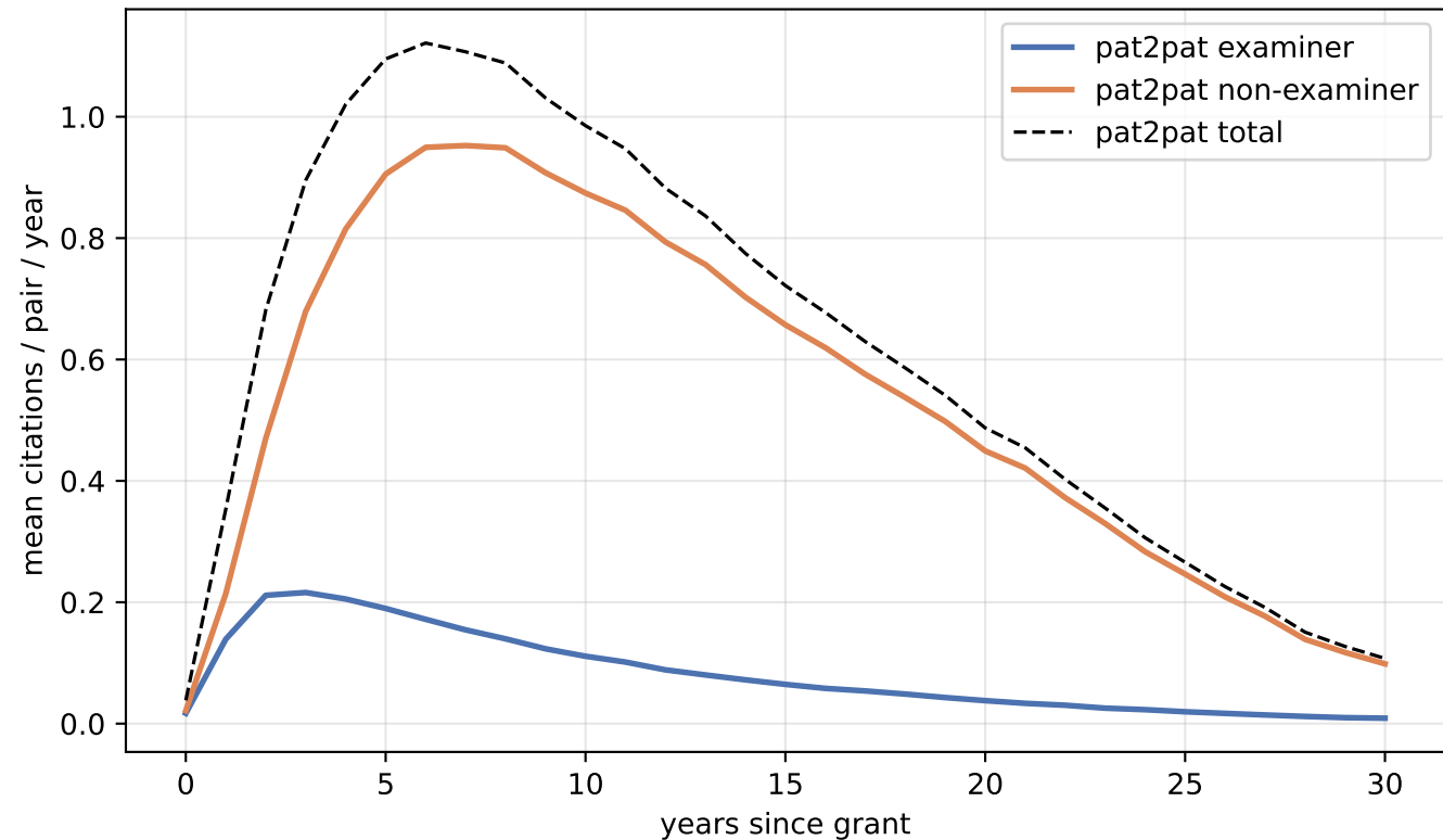
Patent-side citation-age profile
