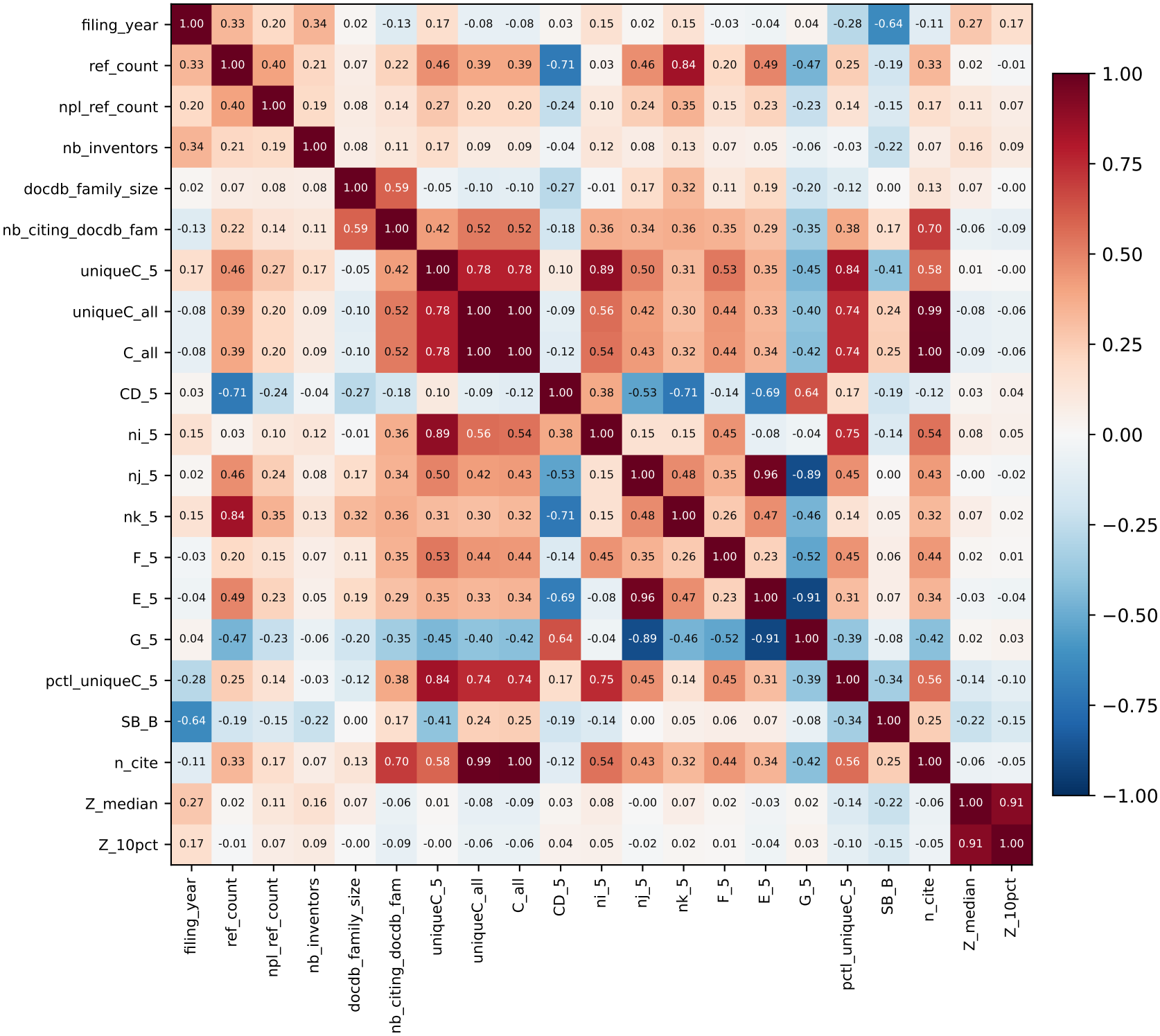
Spearman correlations (500k sample, filing clock)
