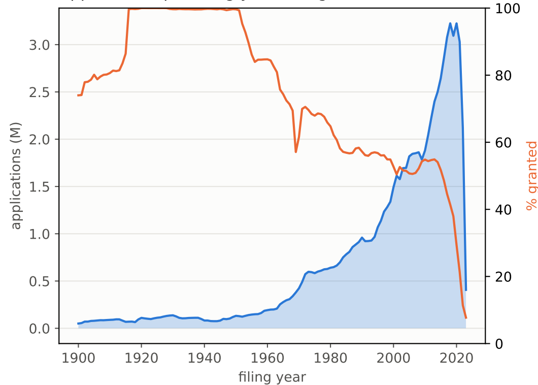
Applications per filing year and grant share
