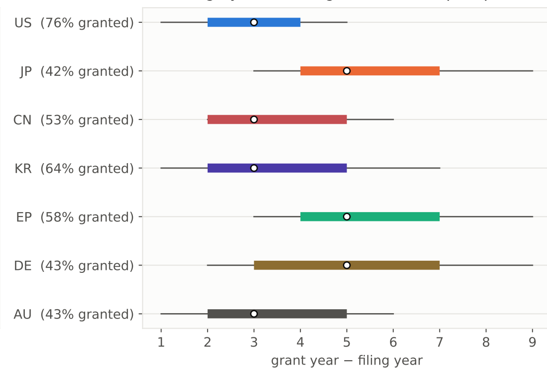
Grant lag by office, filings 1990-2015 (p10-p90, IQR, median)
