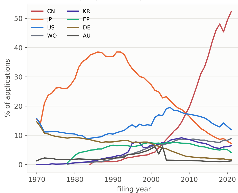
Share of filings by office (top 8 since 1980, to 2021)
