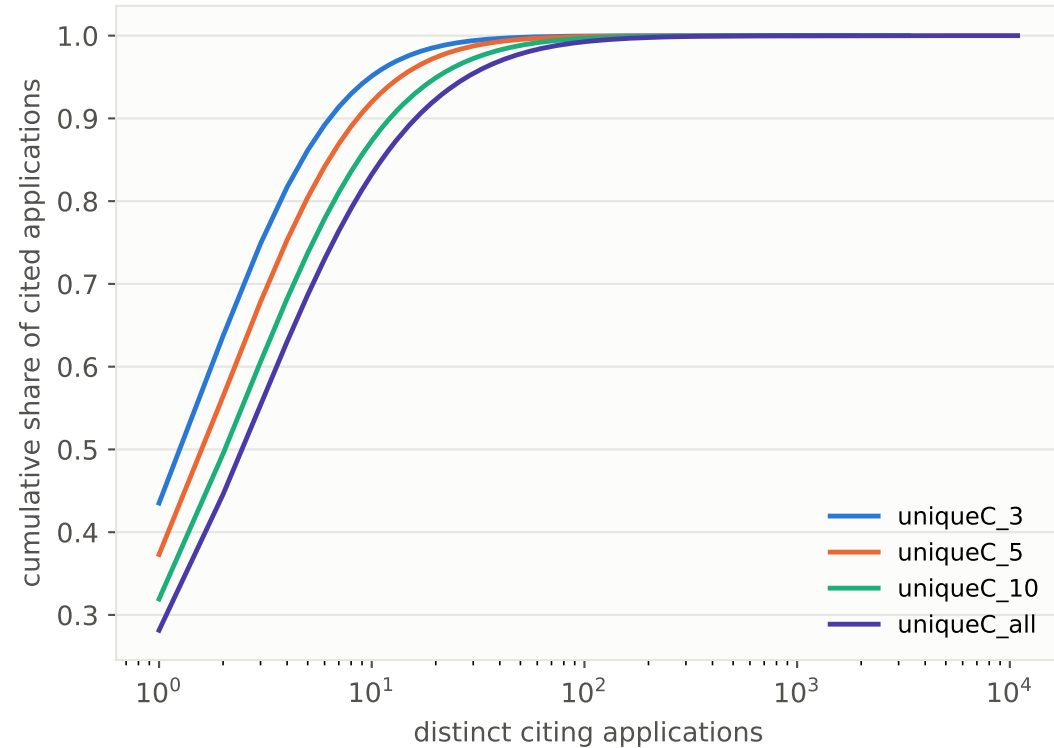
Nested windows
