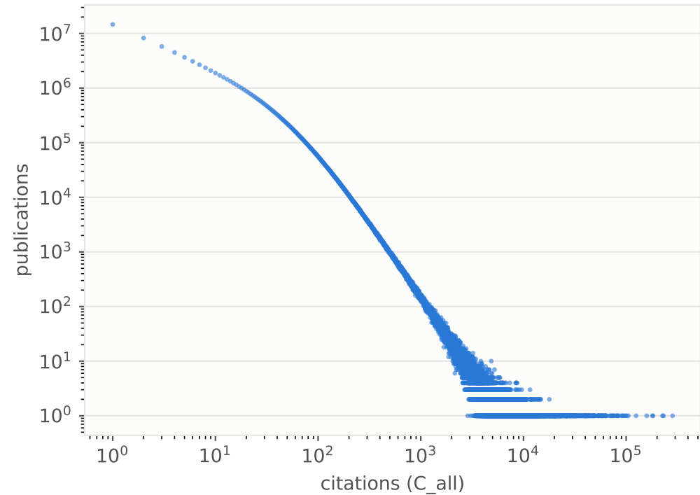
Forward-citation distribution (log-log)
