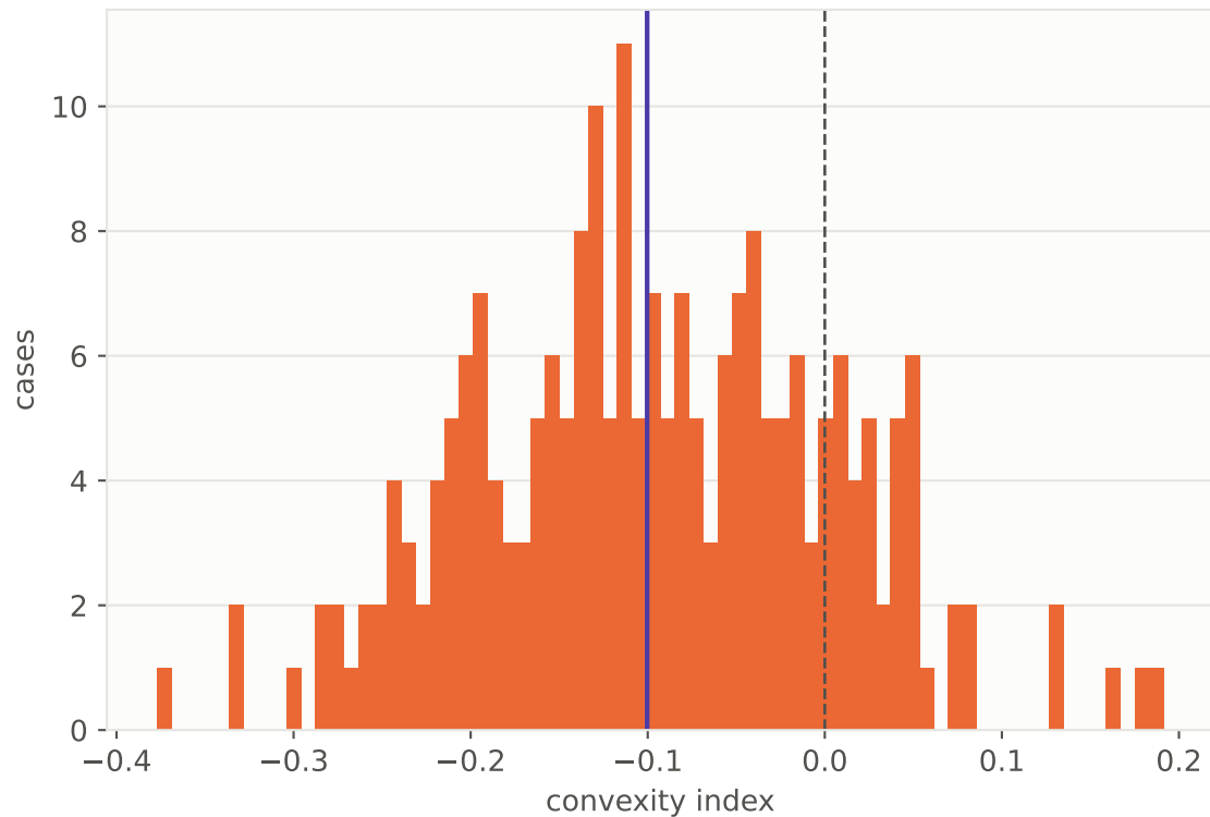
Per-case convexity median -0.1003
