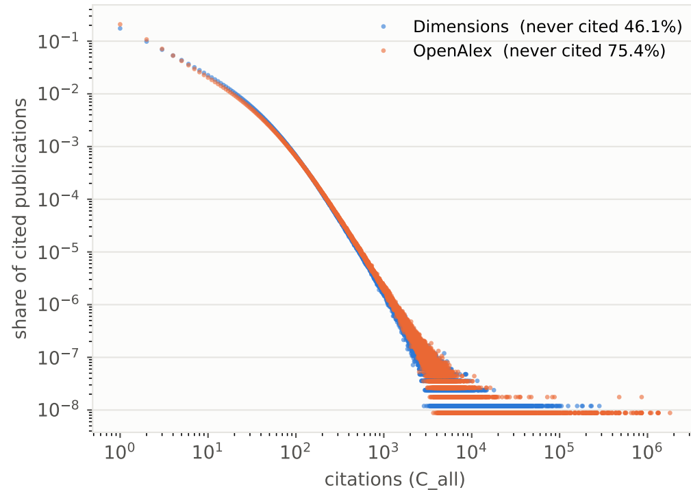
Forward-citation distribution
