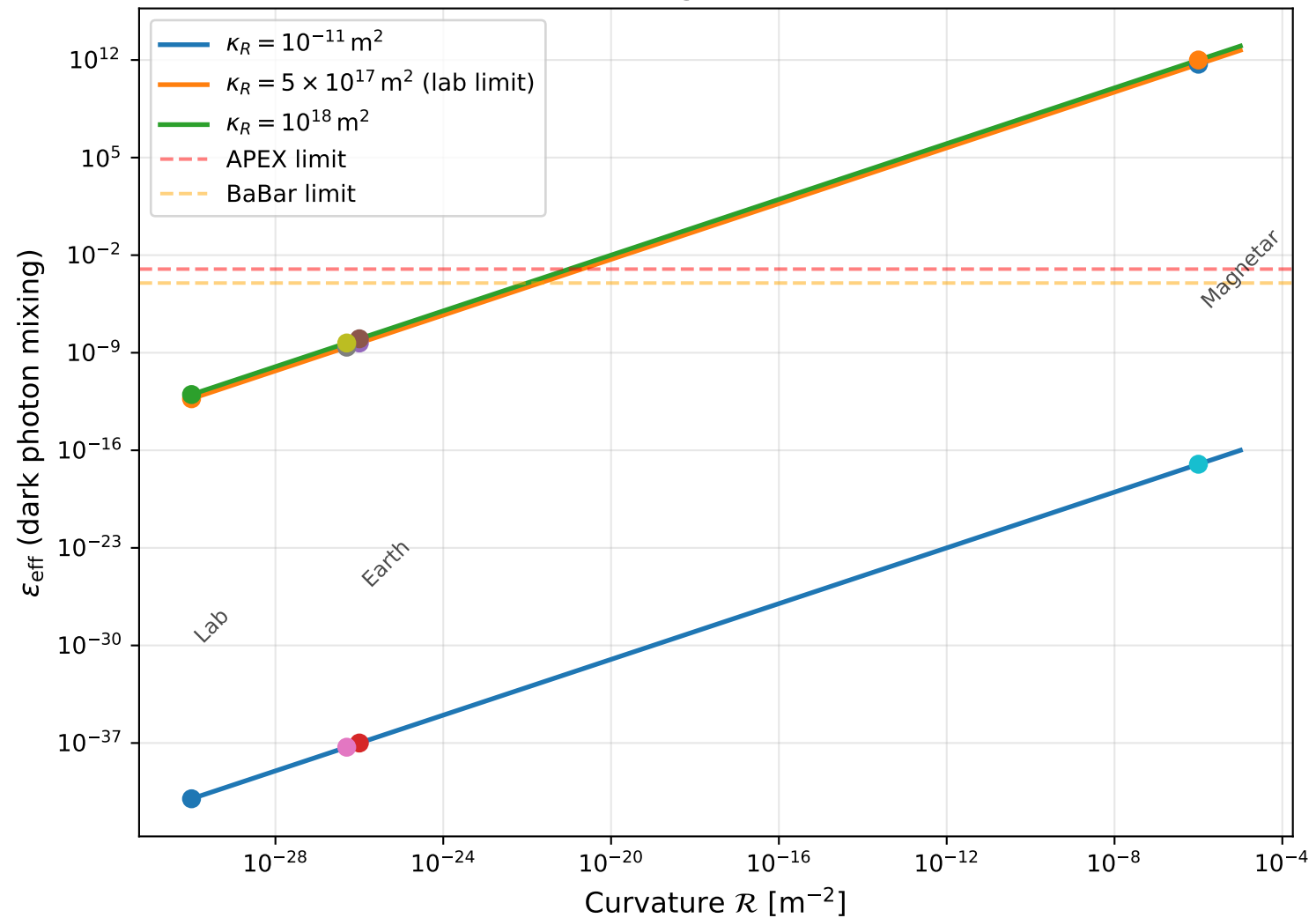
Dark Photon Mixing vs Curvature ( C_\varepsilon = 1 )
