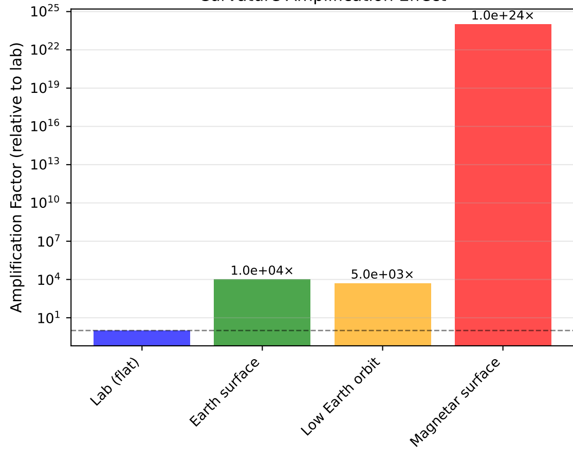
Curvature Amplification Effect
