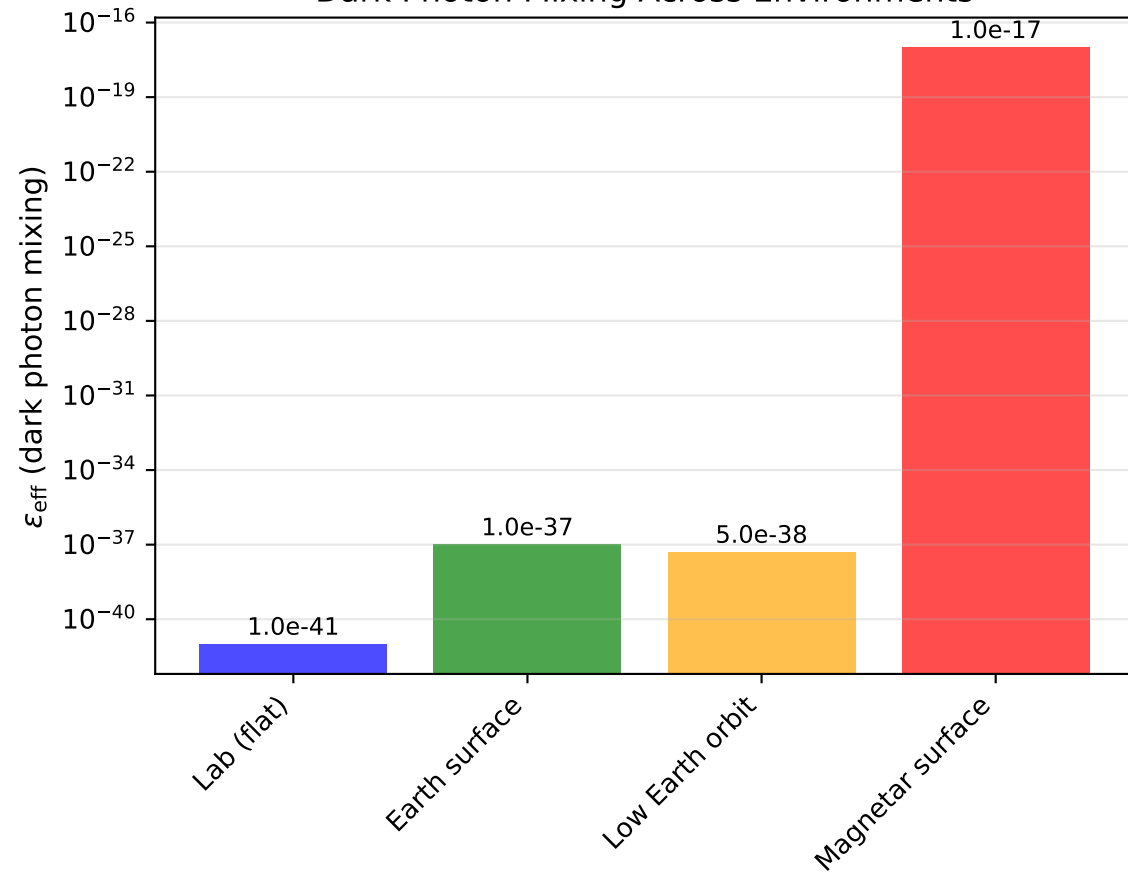
Dark Photon Mixing Across Environments
