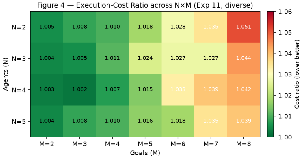
Figure 4: Execution-cost ratio across the N×M grid (Exp 11, diverse distribution, 200 instances/config). Green = near-optimal (ratio →1.0), red = costlier. The worst cell (n2m8, 1.051) is still within ~5% of the exact solver.
