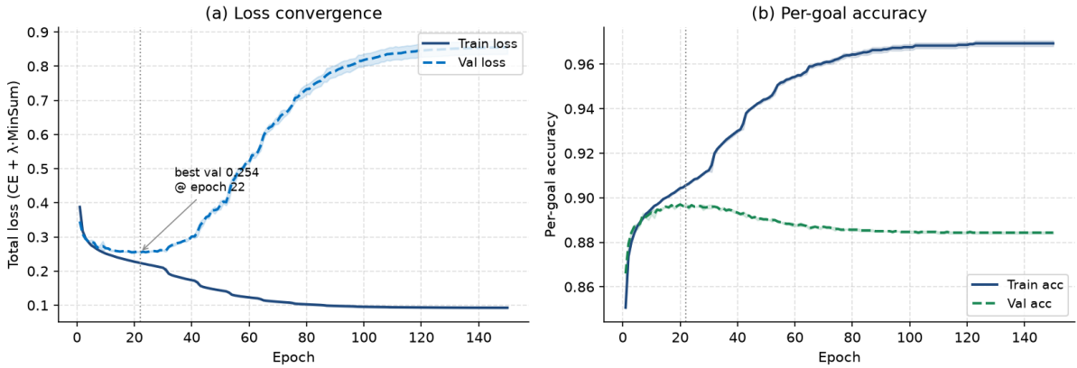
Figure 6: Training convergence of the large model (h128/L6, mean of 3 seeds, \pm 1 std). (a) Total loss: train (solid) keeps falling while validation (dashed) turns upward after its epoch-22 minimum — the checkpoint is taken at that minimum (dotted line). (b) Per-goal accuracy: the train/val gap widens after the same point. Both signatures are textbook overfitting, controlled here by best-val-loss checkpointing.
