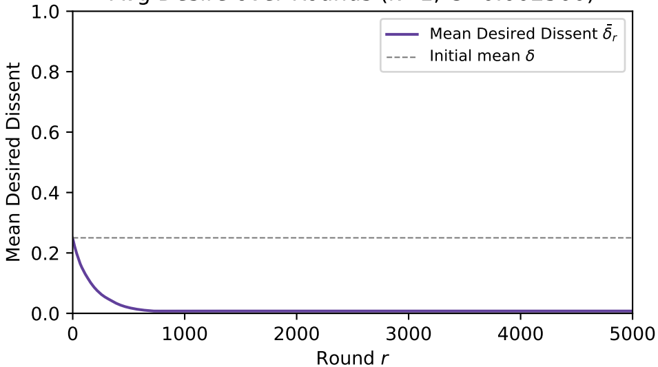
Avg Desire over Rounds ( k=1 , C=0.002500 )
