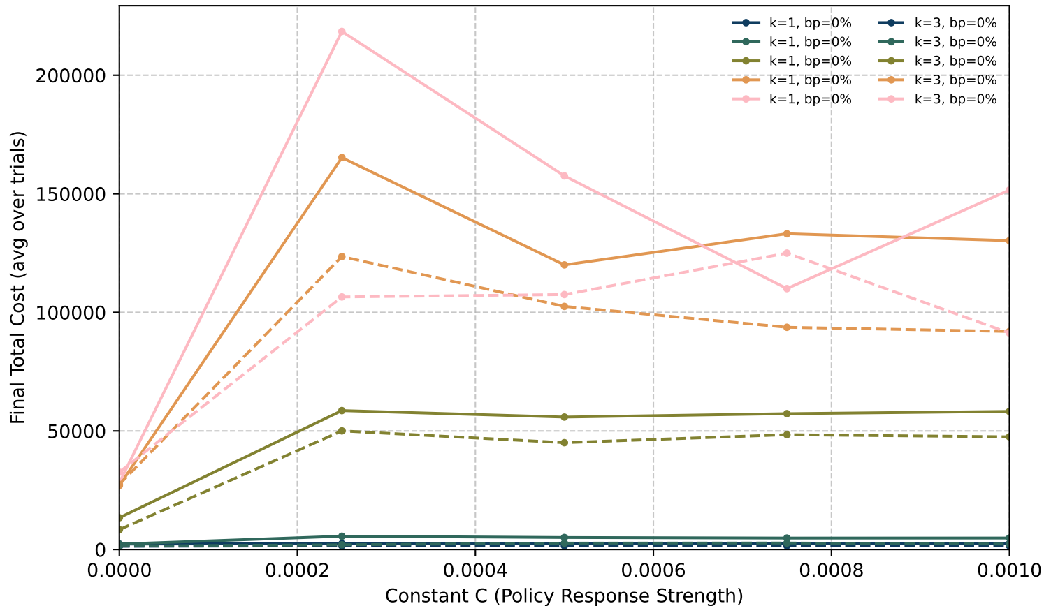
Policy-Responsive Model: C vs Final Cost
