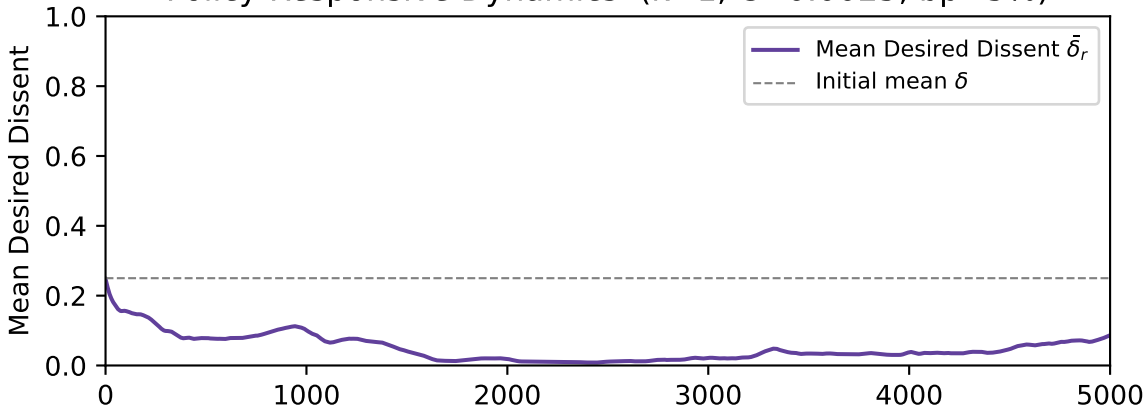
Policy-Responsive Dynamics ( k=1 , C=0.0025 , bp=5\% )
