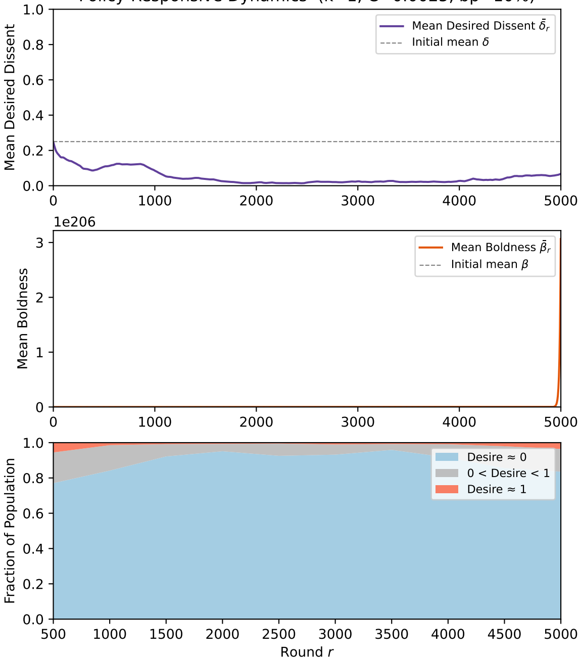
Policy-Responsive Dynamics ( k=1 , C=0.0025 , bp=10\% )
