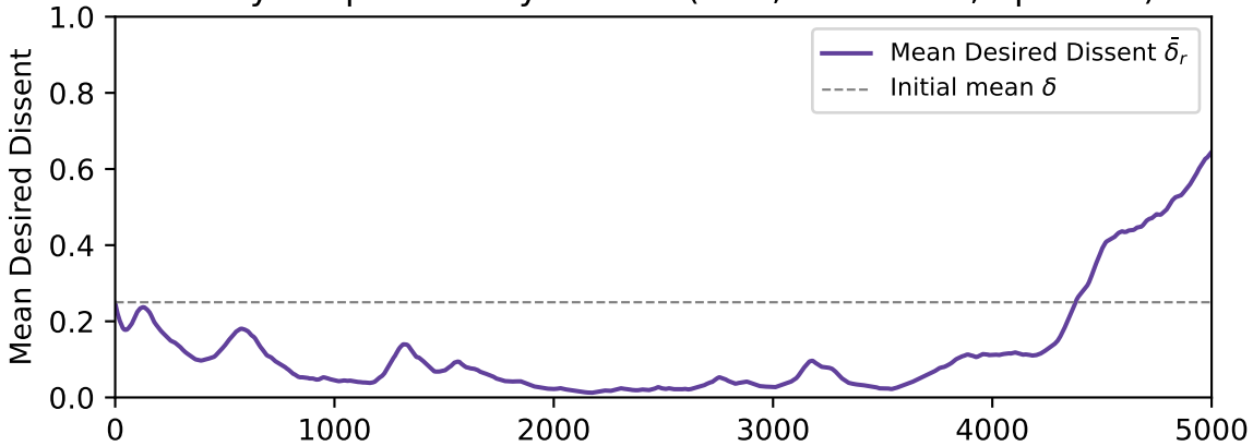
Policy-Responsive Dynamics ( k=3 , C=0.0025 , bp=10\% )
