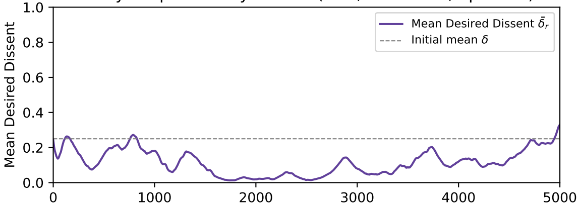
Policy-Responsive Dynamics ( k=3 , C=0.0050 , bp=10\% )
