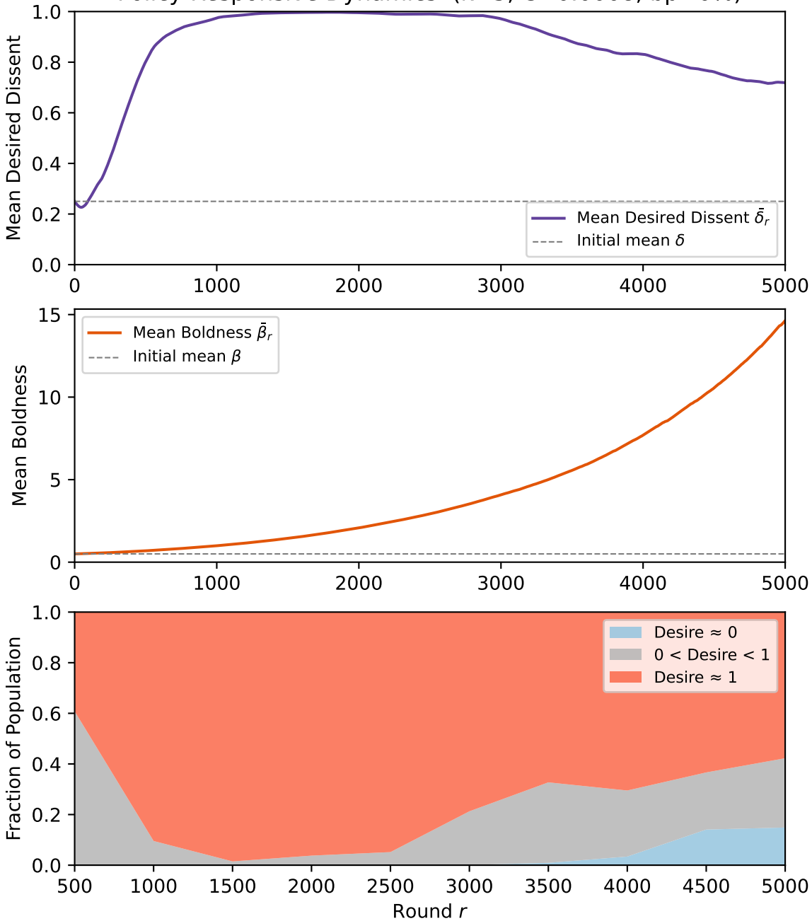
Policy-Responsive Dynamics ( k=3 , C=0.0008 , bp=0\% )
