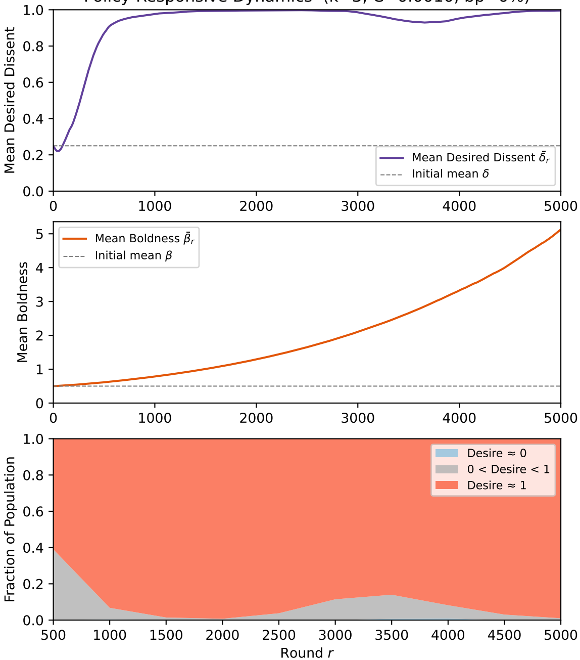
Policy-Responsive Dynamics ( k=3 , C=0.0010 , bp=0\% )
