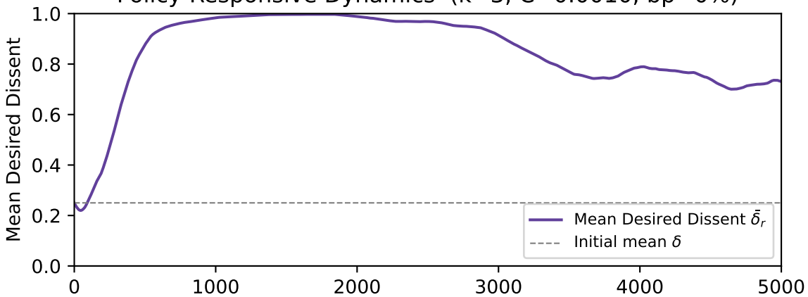
Policy-Responsive Dynamics (k=3, C=0.0010, bp=0%)
